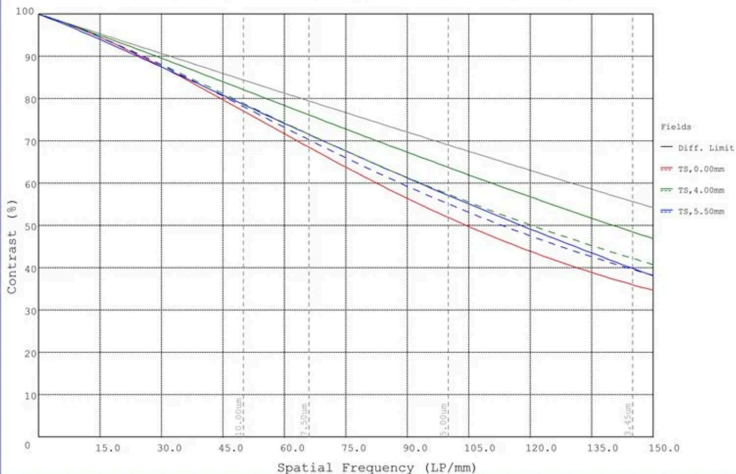
Modulation Transfer Function: 59-870, 16mm
