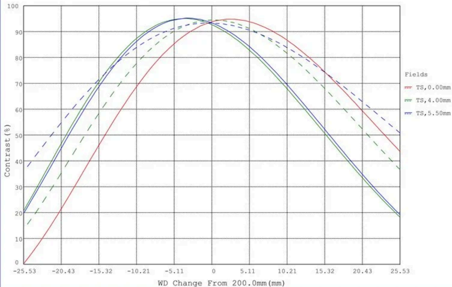
Depth of Field: 59-870, 16mm
