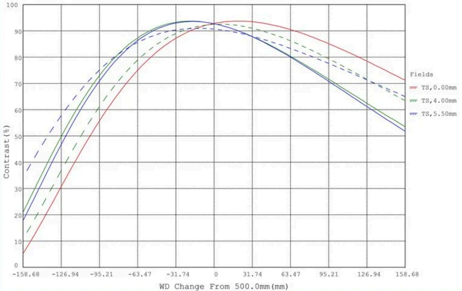
Depth of Field: 59-870, 16mm
