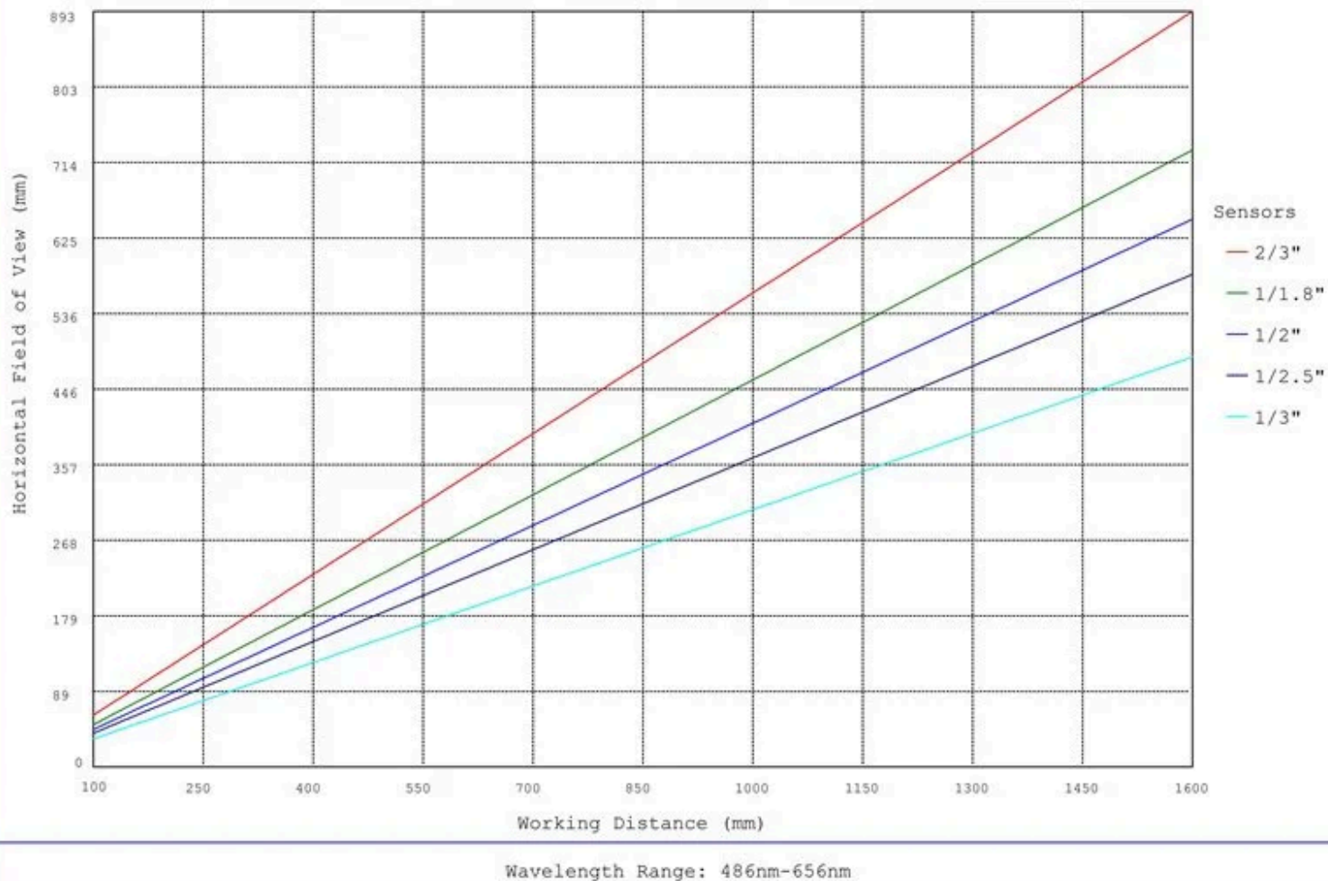
Working Distance vs. Field of View: 59-870, 16mm
