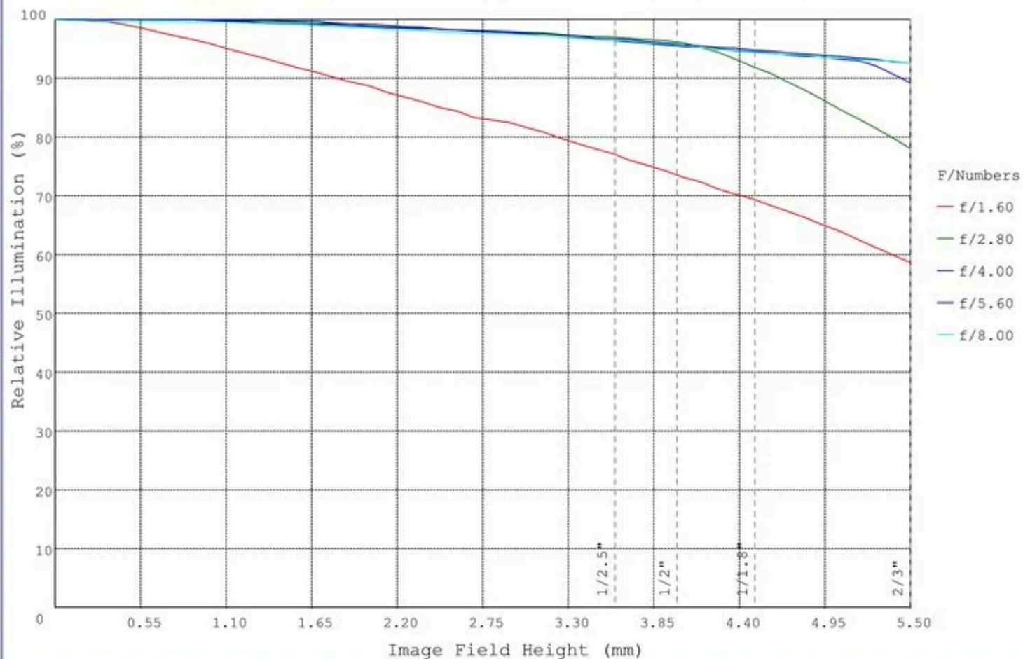
Relative Illumination Plot: 59-870, 16mm
