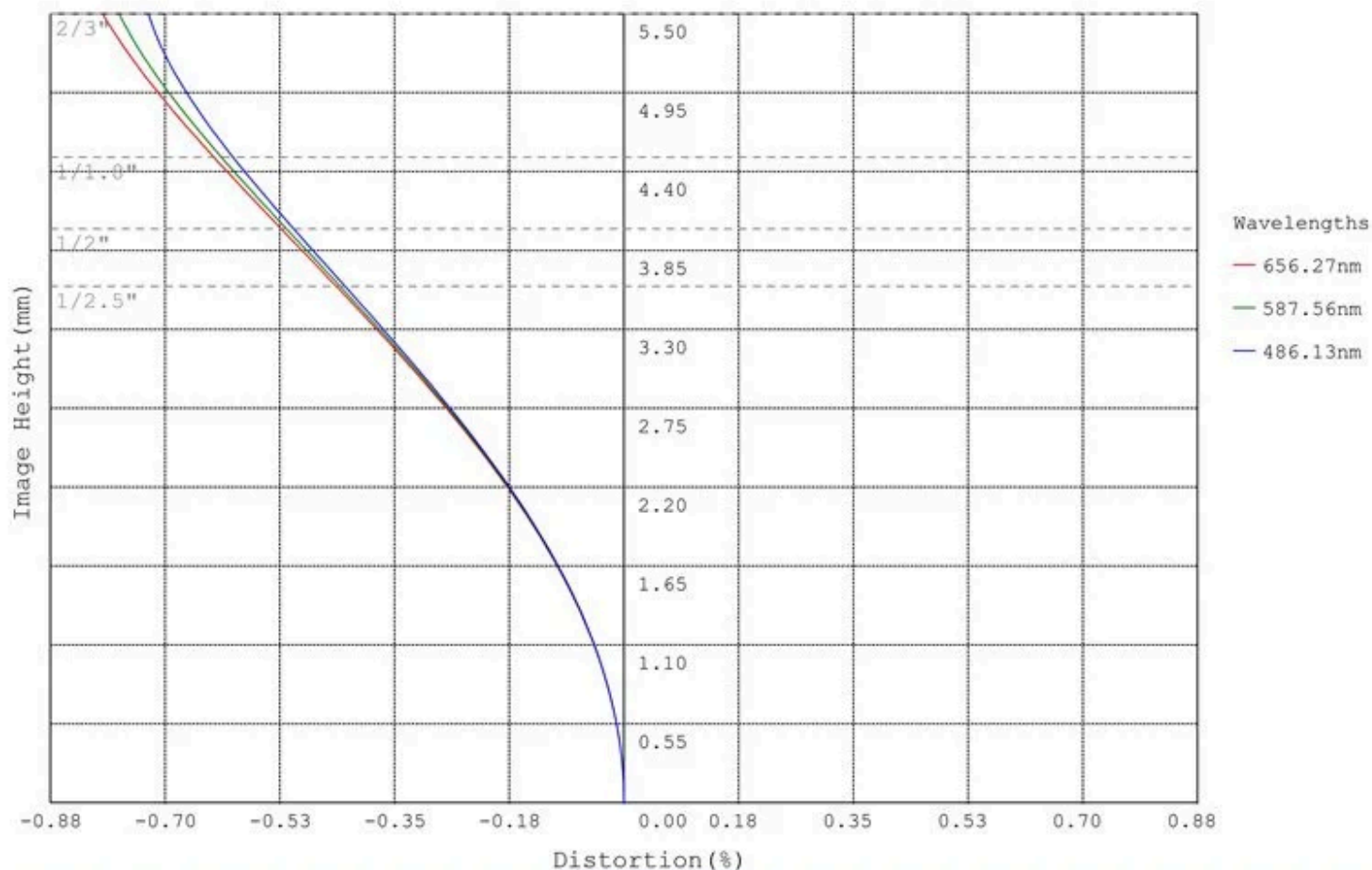
Image Height vs. Distortion: 59-870, 16mm
